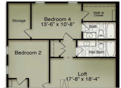
Optional Bedroom 4 with Full Bath and Storage
